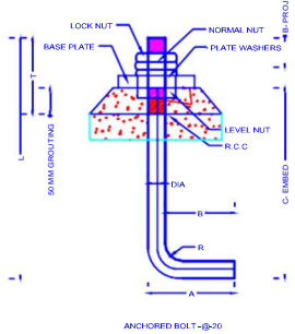
ANCHORED BOLT - Ø-20
