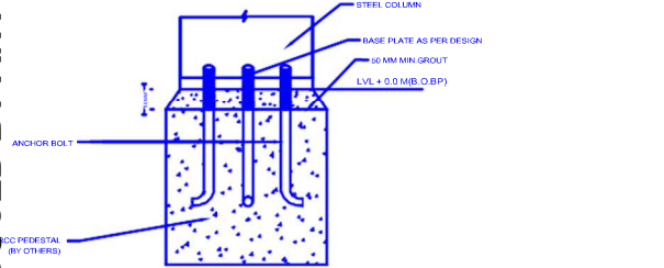
SAMPLE DETAILS OF MINIMUM PEDESTAL REQ FOR PINNED BASE FOR ALL LEAN -TO COLUMN
