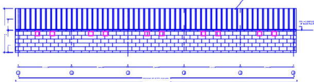
SOWALL SHEETING PLAN FOR FRAME LINE-A
