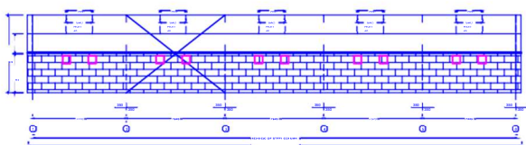
SOWALL FRAMING ELEVATION FOR FRAME LINE-A
