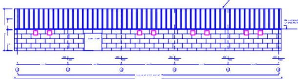
SOWALL SHEETING PLAN FOR FRAME LINE-D
